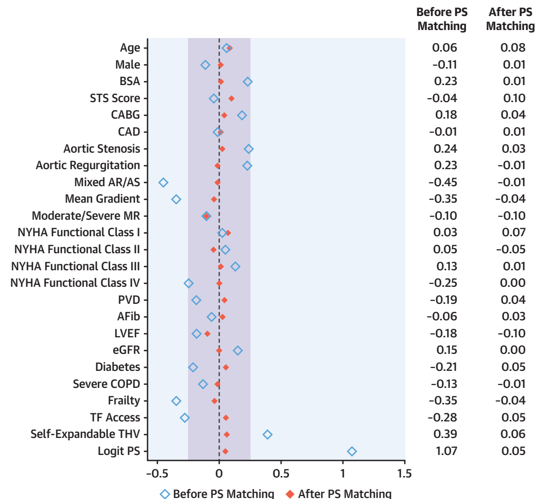
FIGURE 3 Standardized Mean Difference Plot
